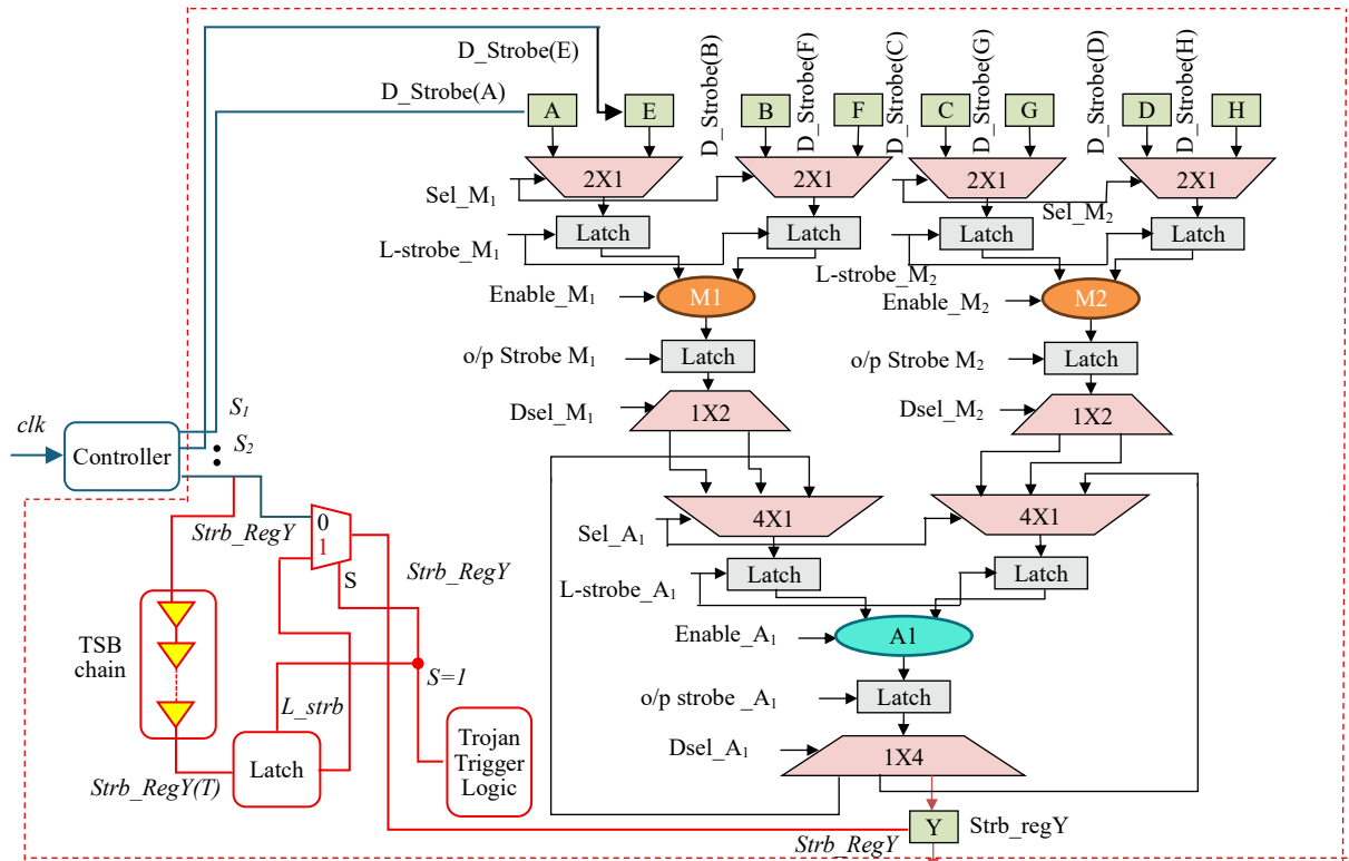
Fig. 2. Details of proposed HLS-aided Trojan infected 4-point DCT IP design (T-DCT)
