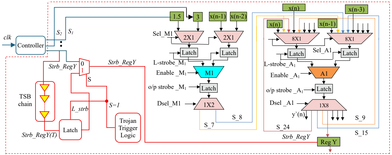
Fig. 4. Details of proposed HLS-aided Trojan infected pacemaker LPF IP design (T-LPF)
