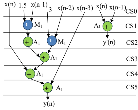
Fig. 3. SDFG of pacemaker LPF IP design
