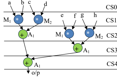
Fig. 1. SDFG of 4-point DCT IP design
